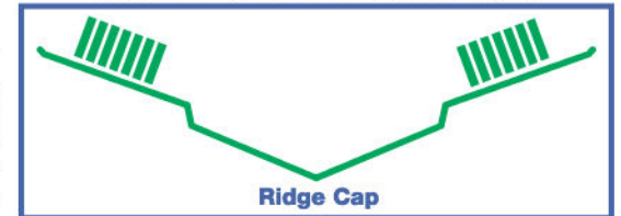
Clean panel of dust & debris. The versatility of the MULTIVENT20 allows installation either onto the ridge cap or the metal roof panel. The roll should sit "up-slope" from the edge of the ridge cap. Double bead adhesive holds MULTIVENT20 securely in place.
