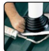
4. Apply sealant
